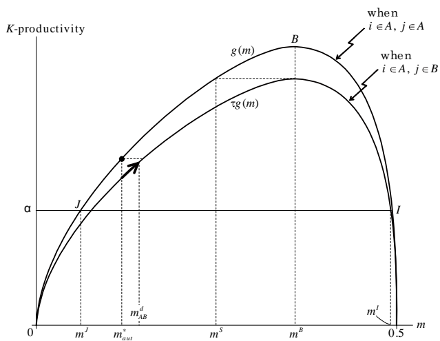
Figure 9: Transition process, Phase 1 (no inter-regional interaction): g(m_{AB}^d) < g(m_{aut}^*)
